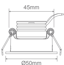
Cutout: Ø45mm - Tilt: 20° Driver fits through cutout hole
