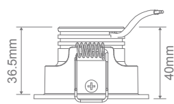
Cutout: Ø45mm - Tilt: 20° Driver fits through cutout hole
