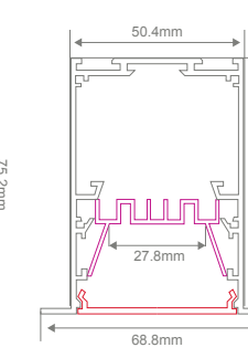
Recessed
