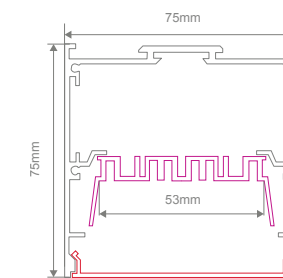
Surface Mounted
